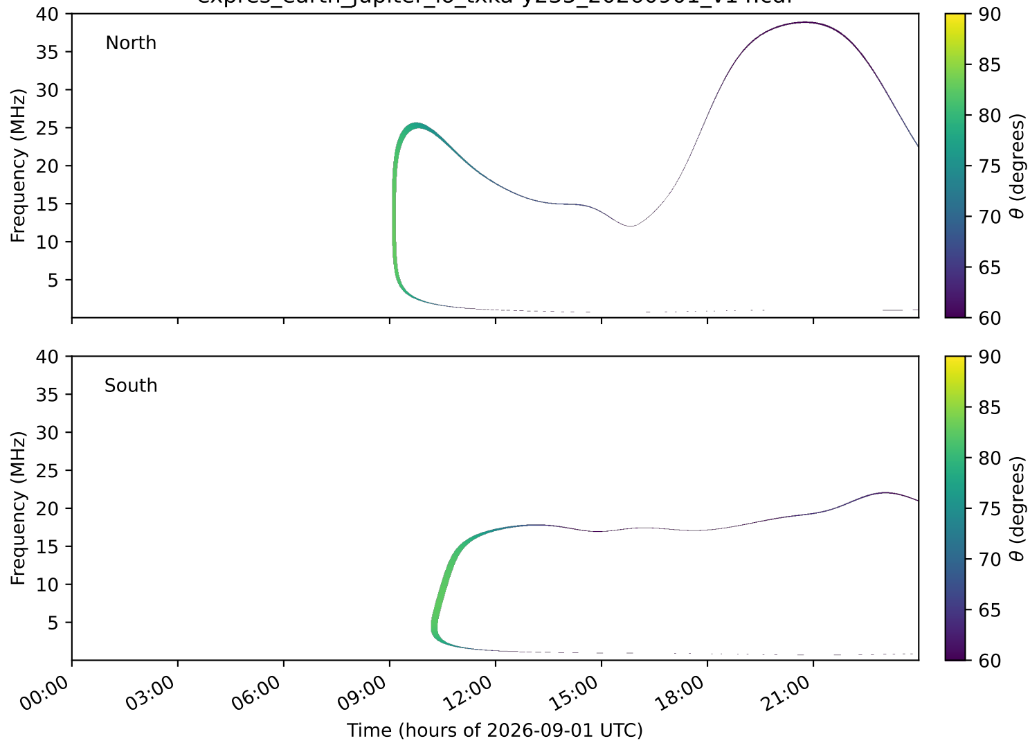
expres_earth_jupiter_io_txka-y235_20260901_v14.cdf
