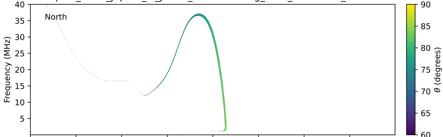
expres_earth_jupiter_io_jrm33_lossc-wid1deg_3kev_20260925_v11.cdf
