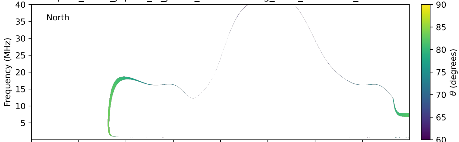
expres_earth_jupiter_io_jrm33_lossc-wid1deg_3kev_20260919_v11.cdf
