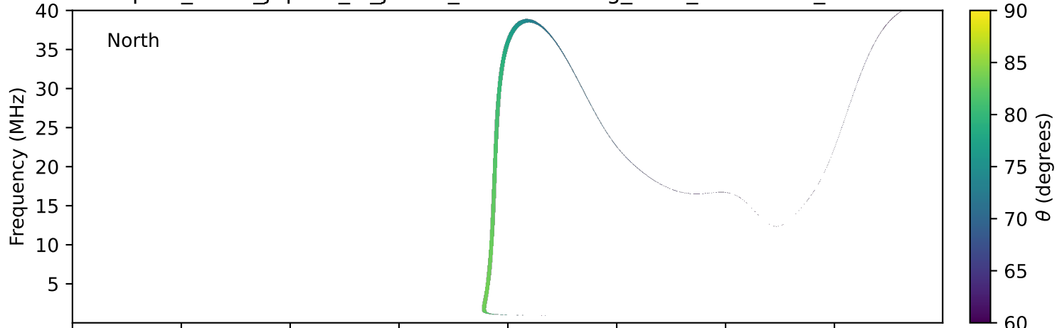
expres_earth_jupiter_io_jrm33_lossc-wid1deg_3kev_20260917_v11.cdf
