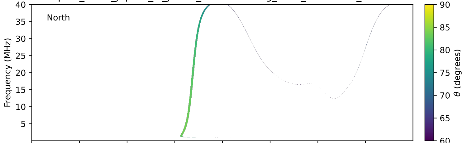
expres_earth_jupiter_io_jrm33_lossc-wid1deg_3kev_20260910_v11.cdf
