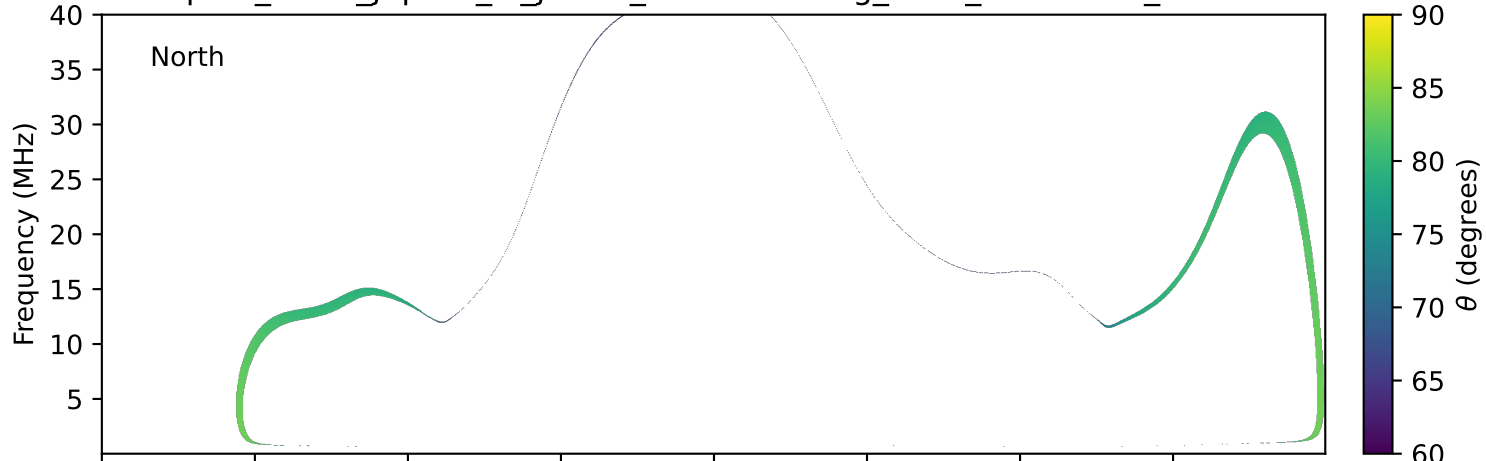
expres_earth_jupiter_io_jrm33_lossc-wid1deg_3kev_20260903_v11.cdf
