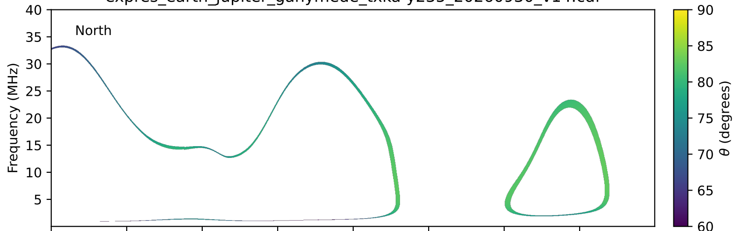
expres_earth_jupiter_ganymede_txka-y235_20260930_v14.cdf
