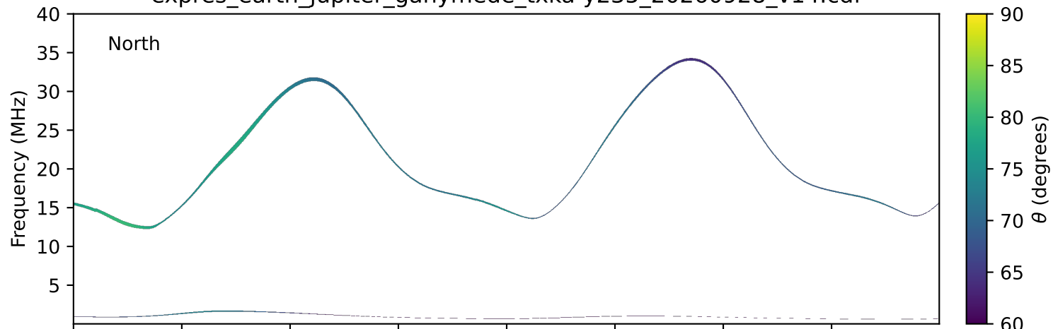
expres_earth_jupiter_ganymede_txka-y235_20260928_v14.cdf
