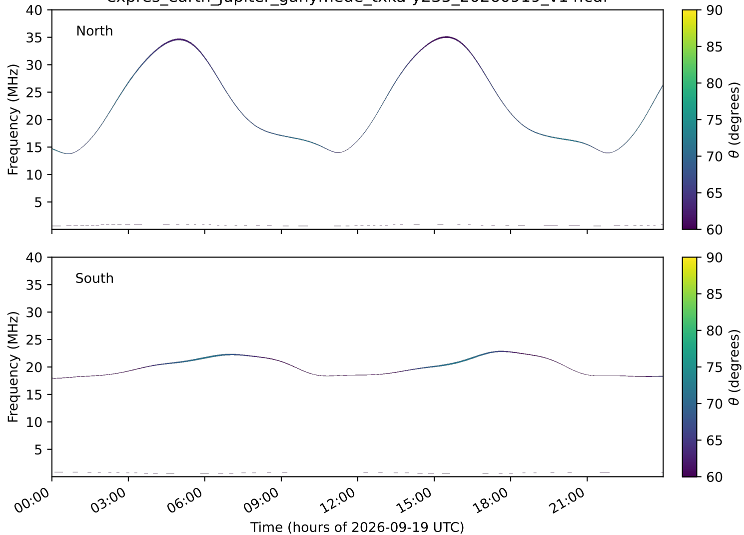
expres_earth_jupiter_ganymede_txka-y235_20260919_v14.cdf
