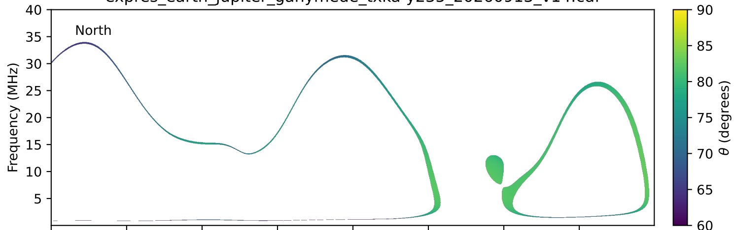
expres_earth_jupiter_ganymede_txka-y235_20260913_v14.cdf
