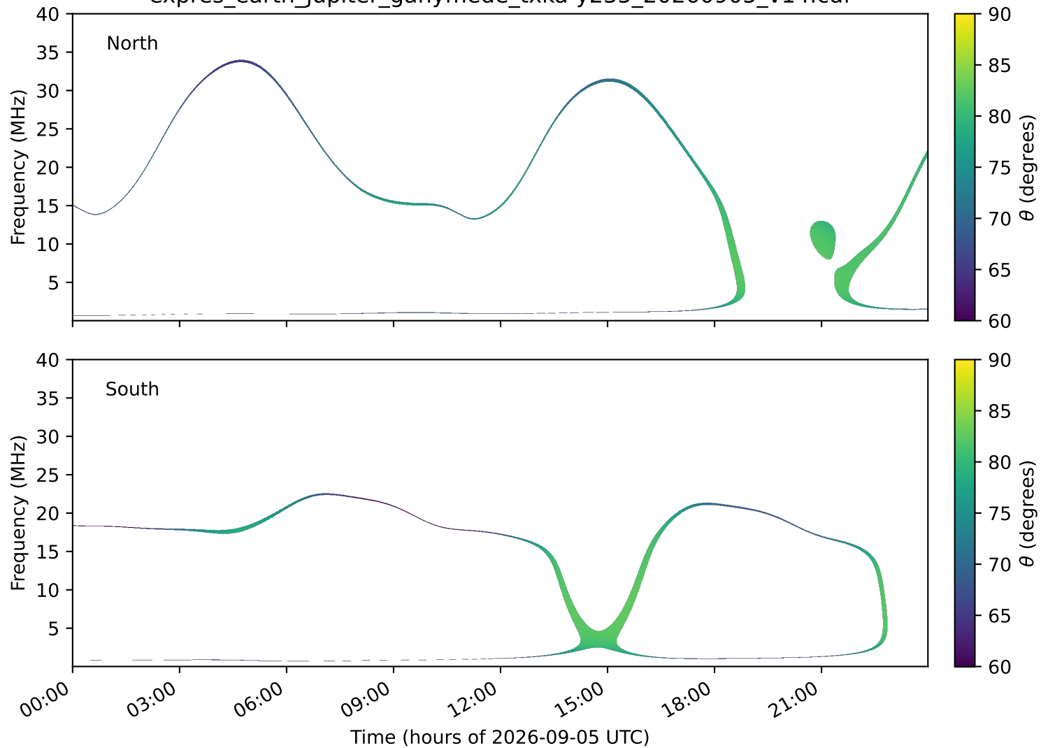
expres_earth_jupiter_ganymede_txka-y235_20260905_v14.cdf
