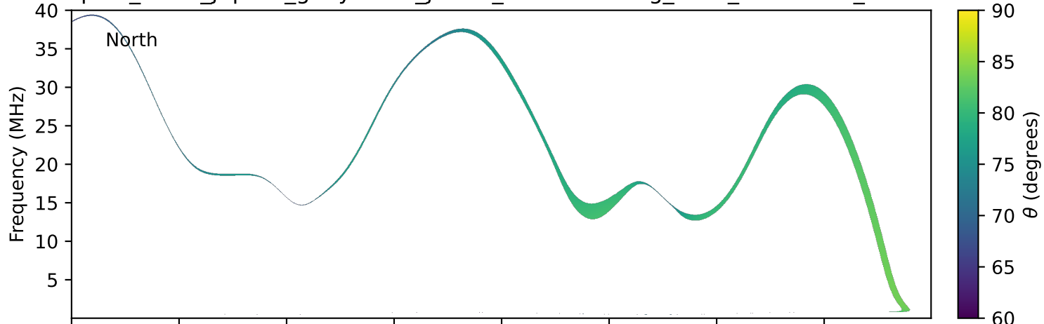
expres_earth_jupiter_ganymede_jrm33_lossc-wid1deg_3kev_20260930_v11.cdf
