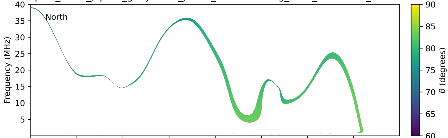
expres_earth_jupiter_ganymede_jrm33_lossc-wid1deg_3kev_20260923_v11.cdf
