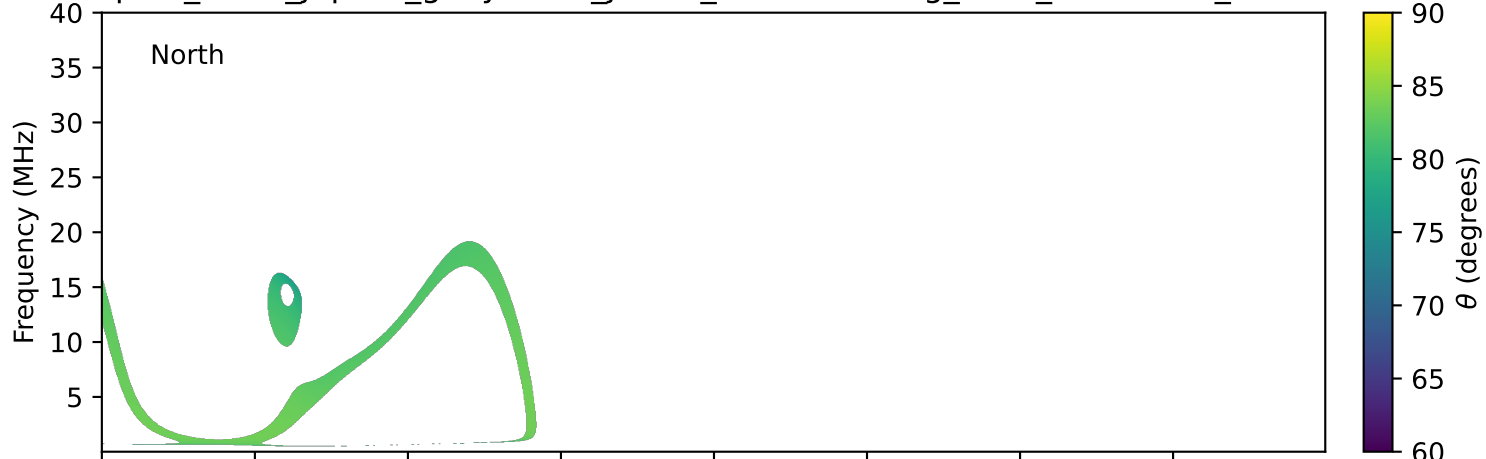
expres_earth_jupiter_ganymede_jrm33_lossc-wid1deg_3kev_20260914_v11.cdf
