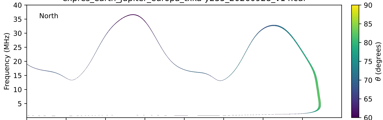
expres_earth_jupiter_europa_txka-y235_20260928_v14.cdf
