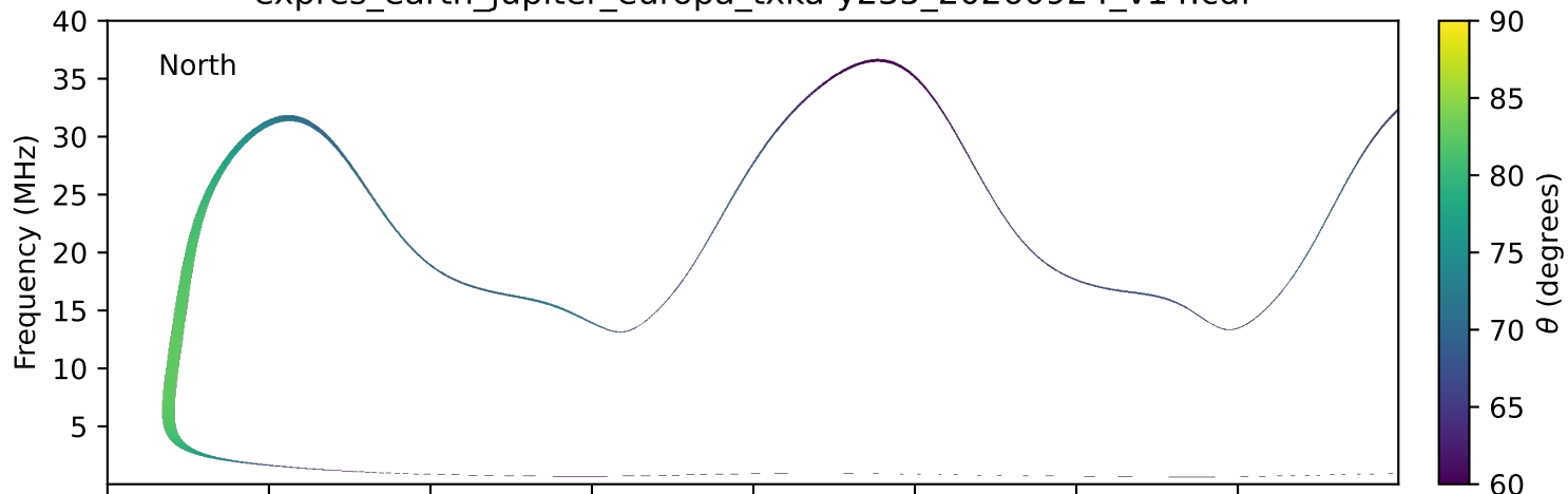
expres_earth_jupiter_europa_txka-y235_20260924_v14.cdf
