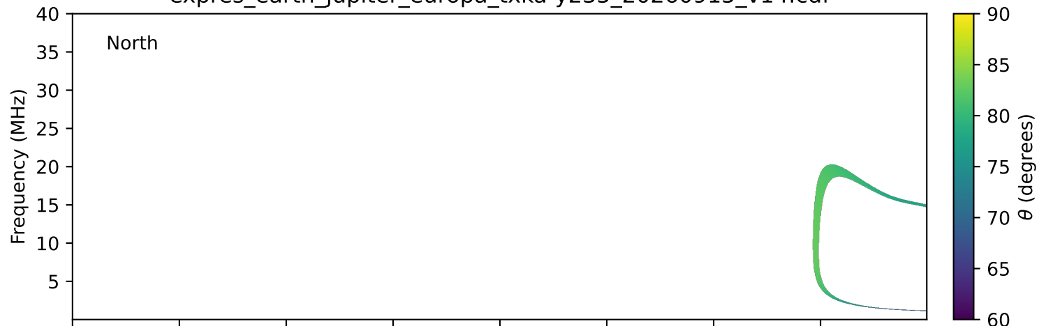
expres_earth_jupiter_europa_txka-y235_20260915_v14.cdf
