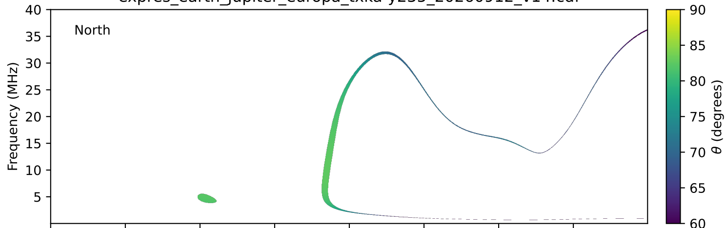
expres_earth_jupiter_europa_txka-y235_20260912_v14.cdf
