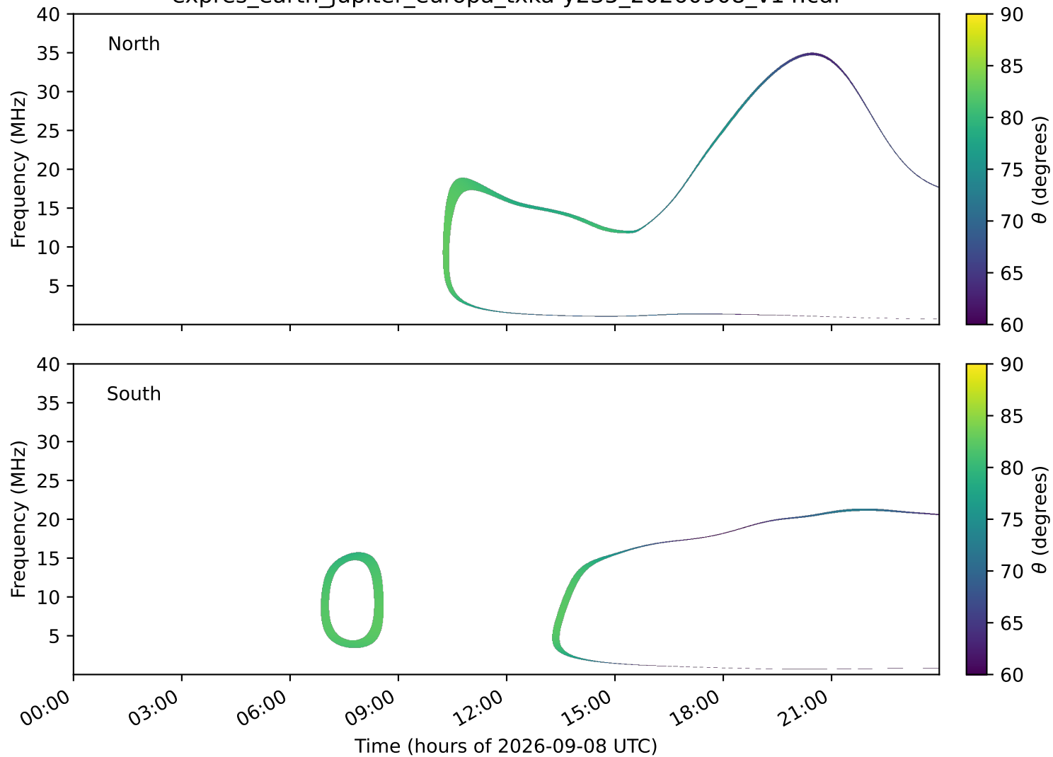
expres_earth_jupiter_europa_txka-y235_20260908_v14.cdf
