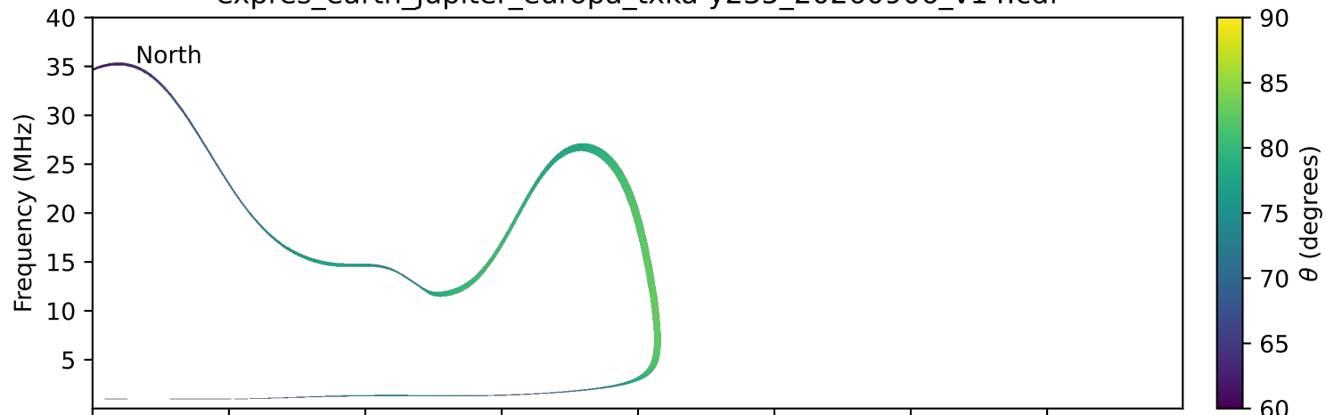
expres_earth_jupiter_europa_txka-y235_20260906_v14.cdf
