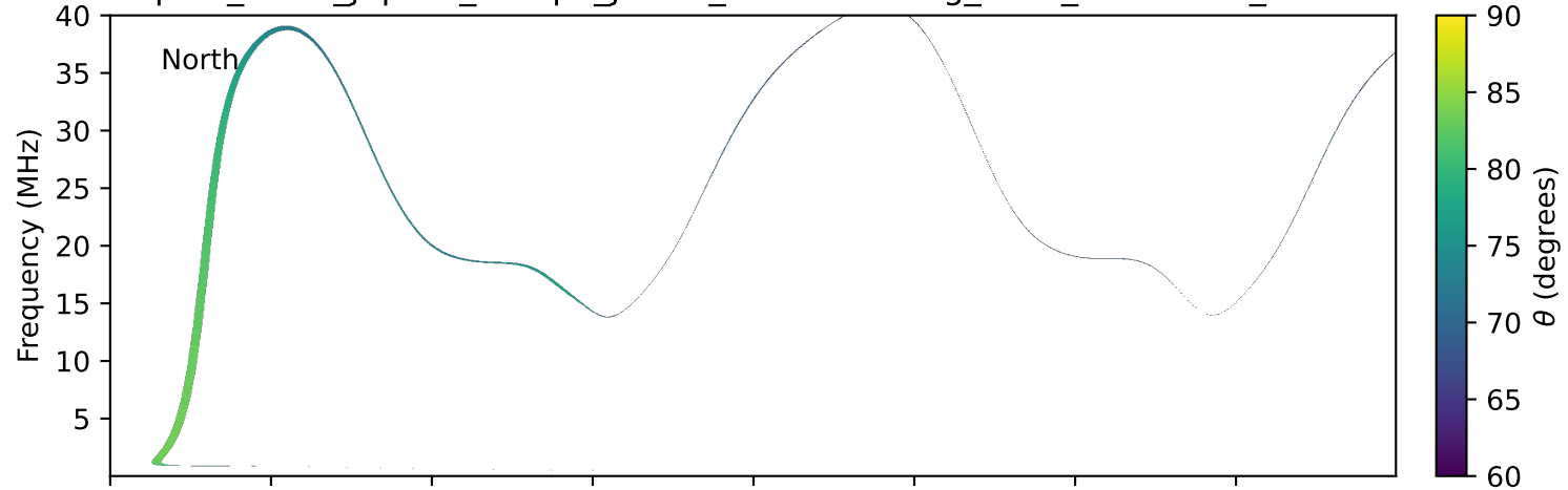
expres_earth_jupiter_europa_jrm33_lossc-wid1deg_3kev_20260924_v11.cdf
