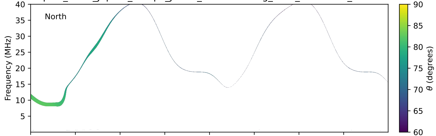
expres_earth_jupiter_europa_jrm33_lossc-wid1deg_3kev_20260916_v11.cdf
