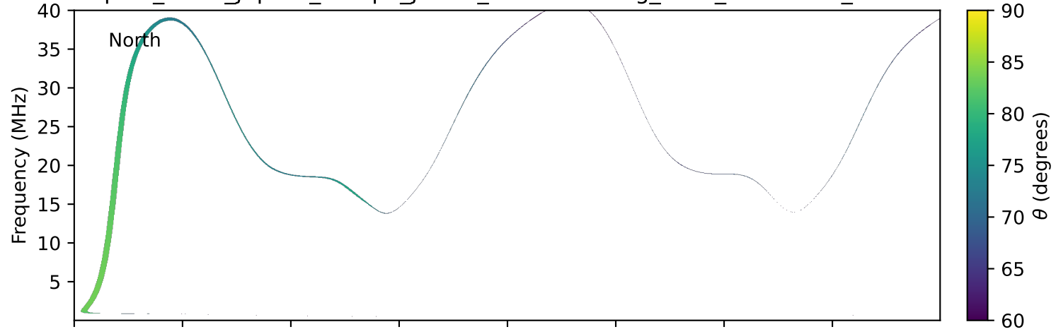
expres_earth_jupiter_europa_jrm33_lossc-wid1deg_3kev_20260905_v11.cdf
