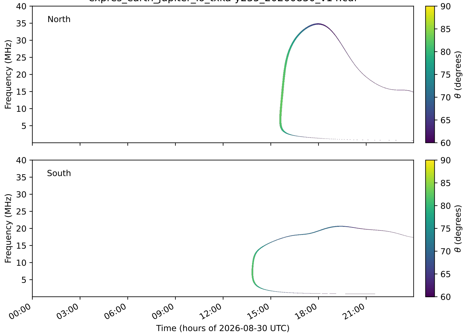
expres_earth_jupiter_io_txka-y235_20260830_v14.cdf
