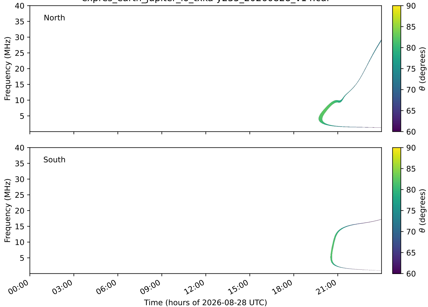
expres_earth_jupiter_io_txka-y235_20260828_v14.cdf
