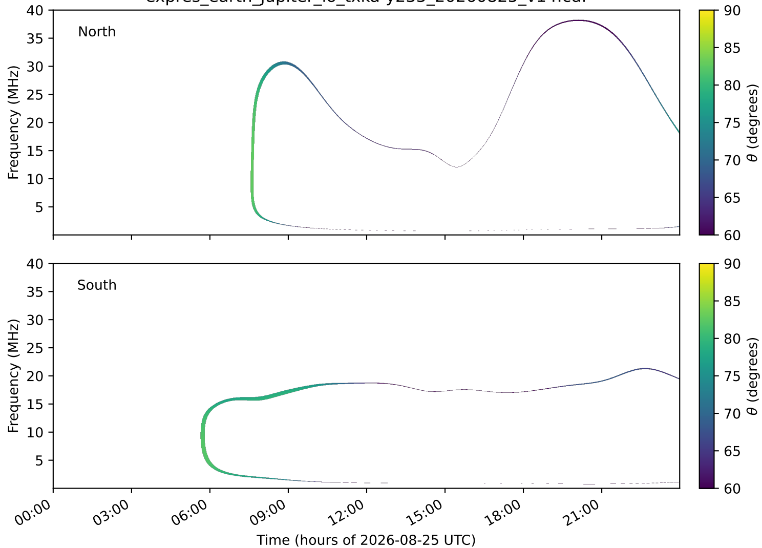
expres_earth_jupiter_io_txka-y235_20260825_v14.cdf
