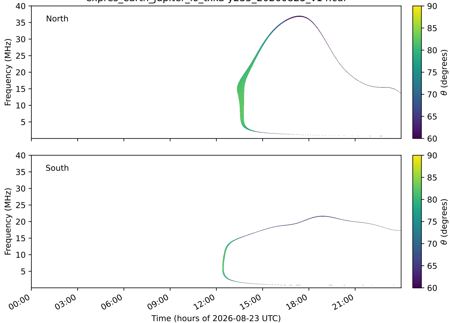
expres_earth_jupiter_io_txka-y235_20260823_v14.cdf
