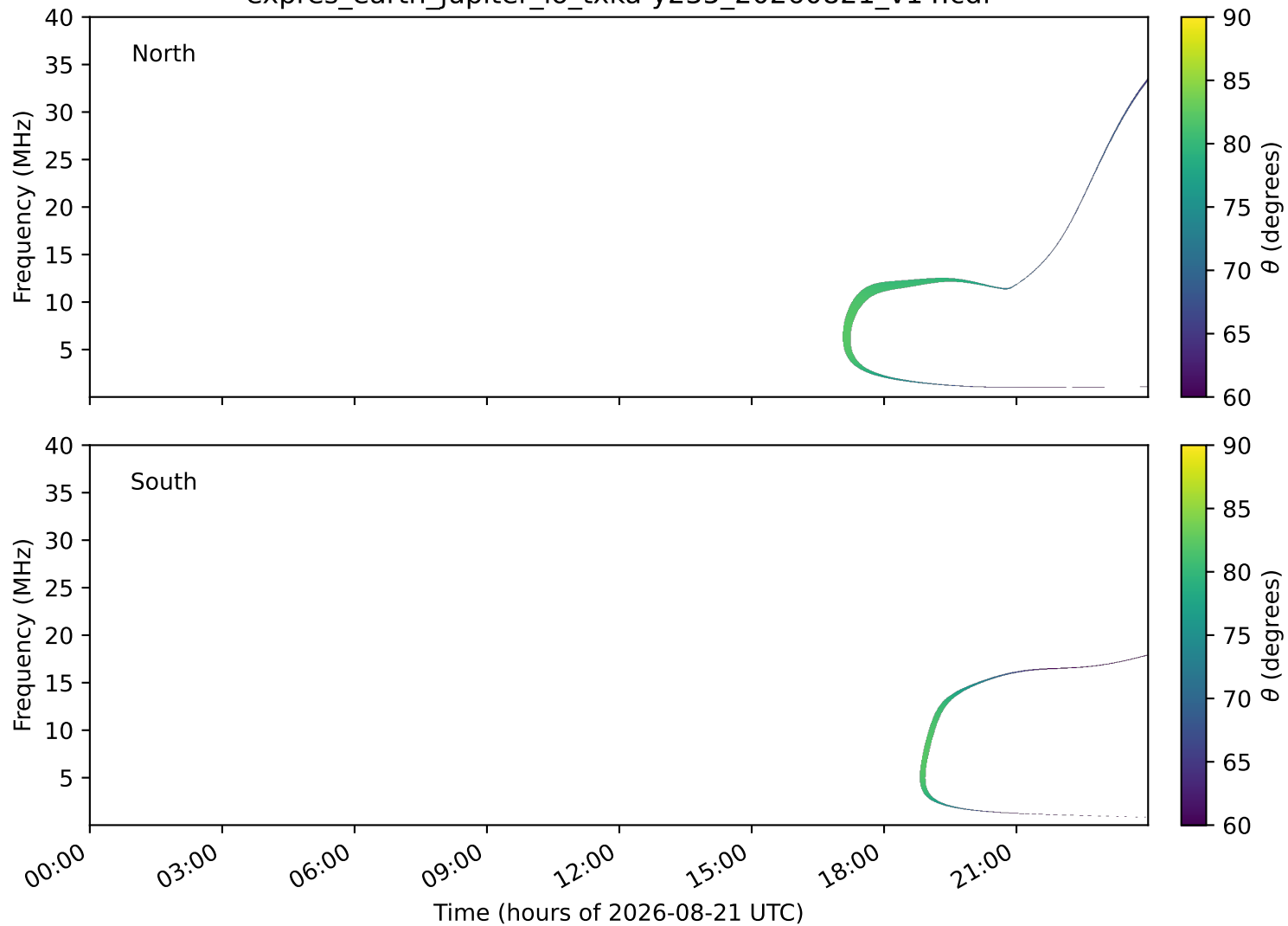
expres_earth_jupiter_io_txka-y235_20260821_v14.cdf
