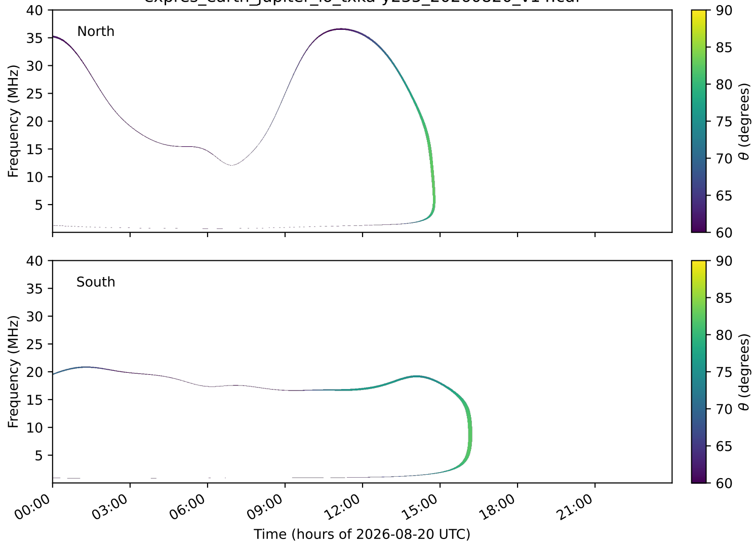
expres_earth_jupiter_io_txka-y235_20260820_v14.cdf
