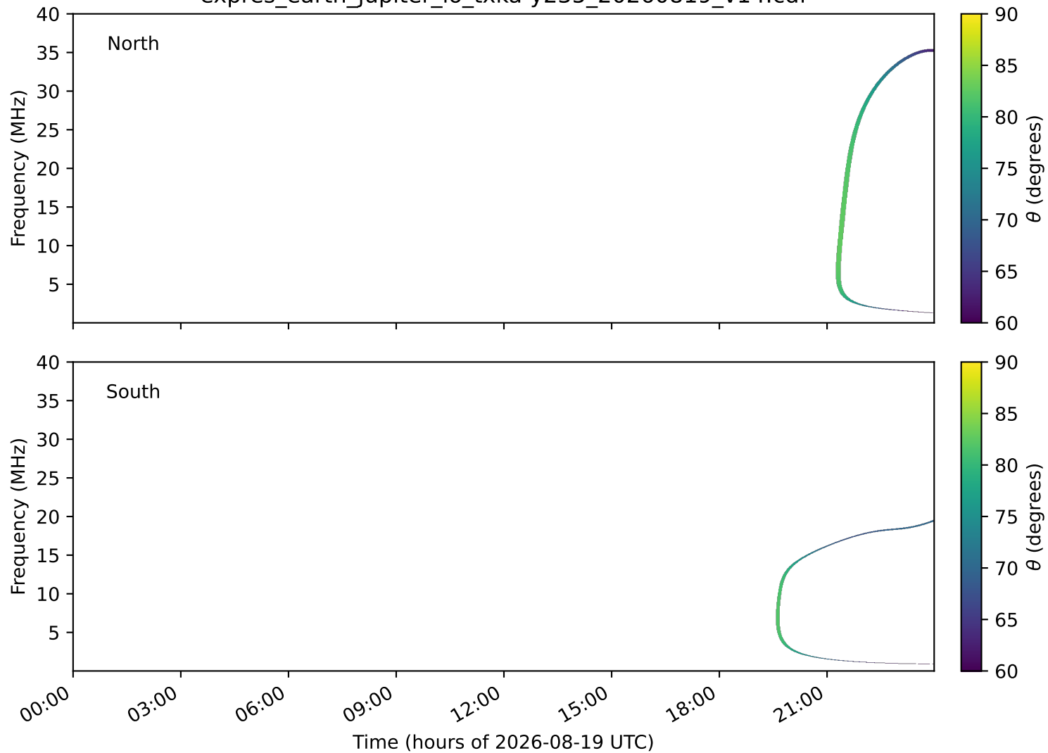
expres_earth_jupiter_io_txka-y235_20260819_v14.cdf
