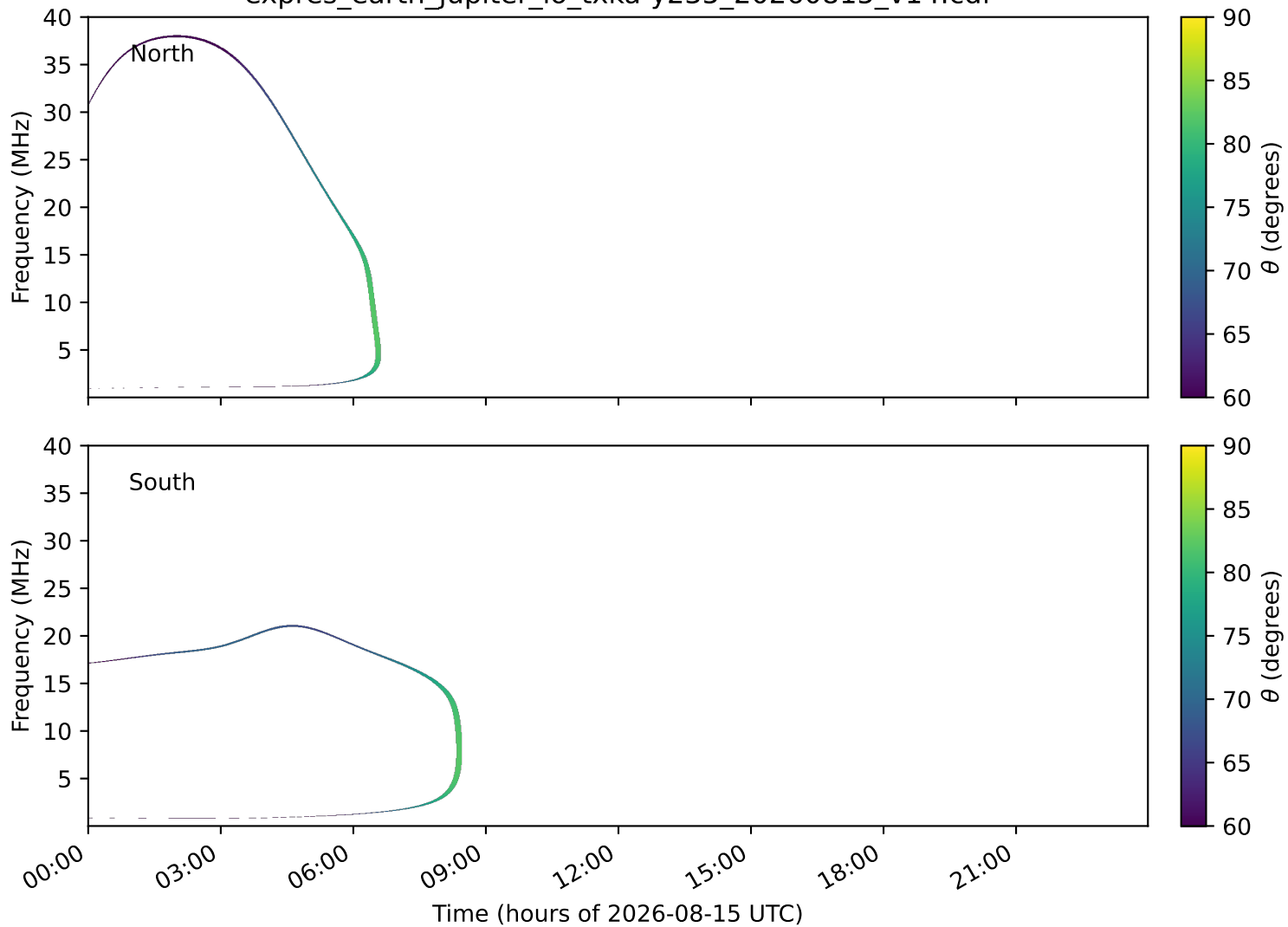
expres_earth_jupiter_io_txka-y235_20260815_v14.cdf
