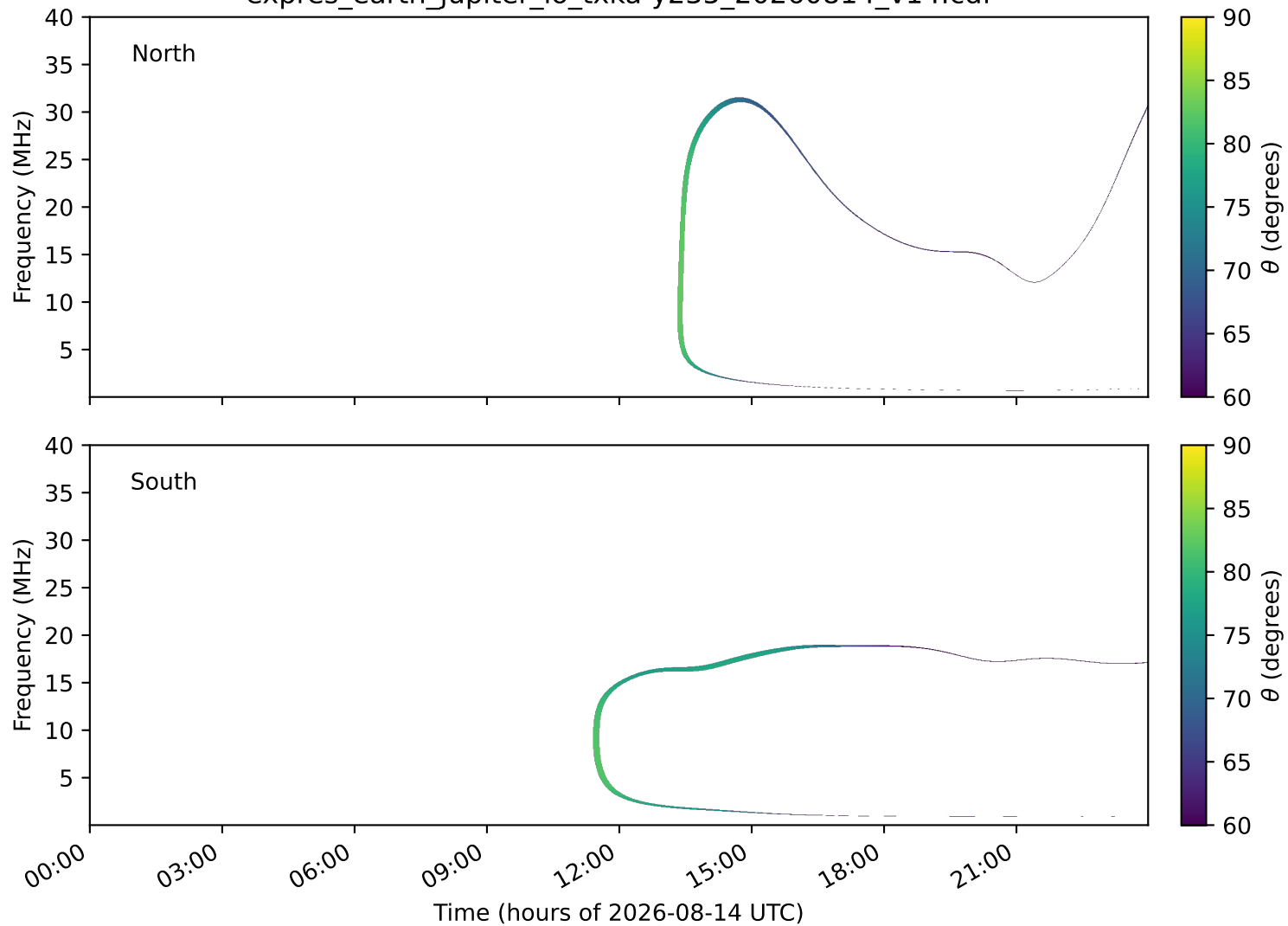
expres_earth_jupiter_io_txka-y235_20260814_v14.cdf
