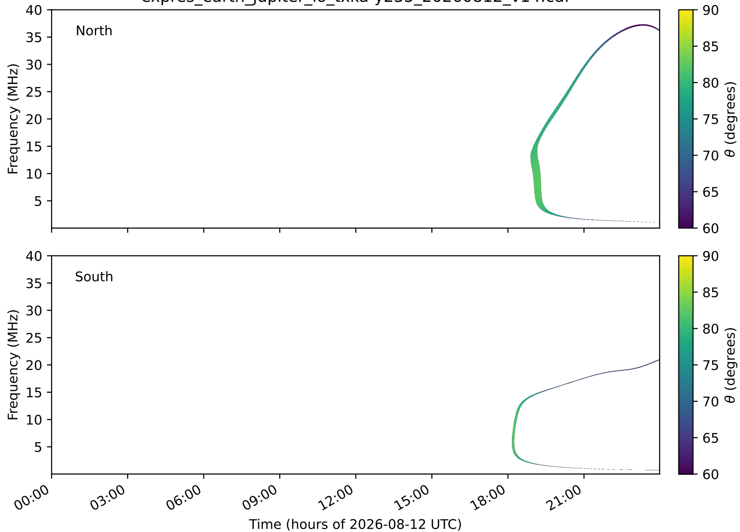
expres_earth_jupiter_io_txka-y235_20260812_v14.cdf
