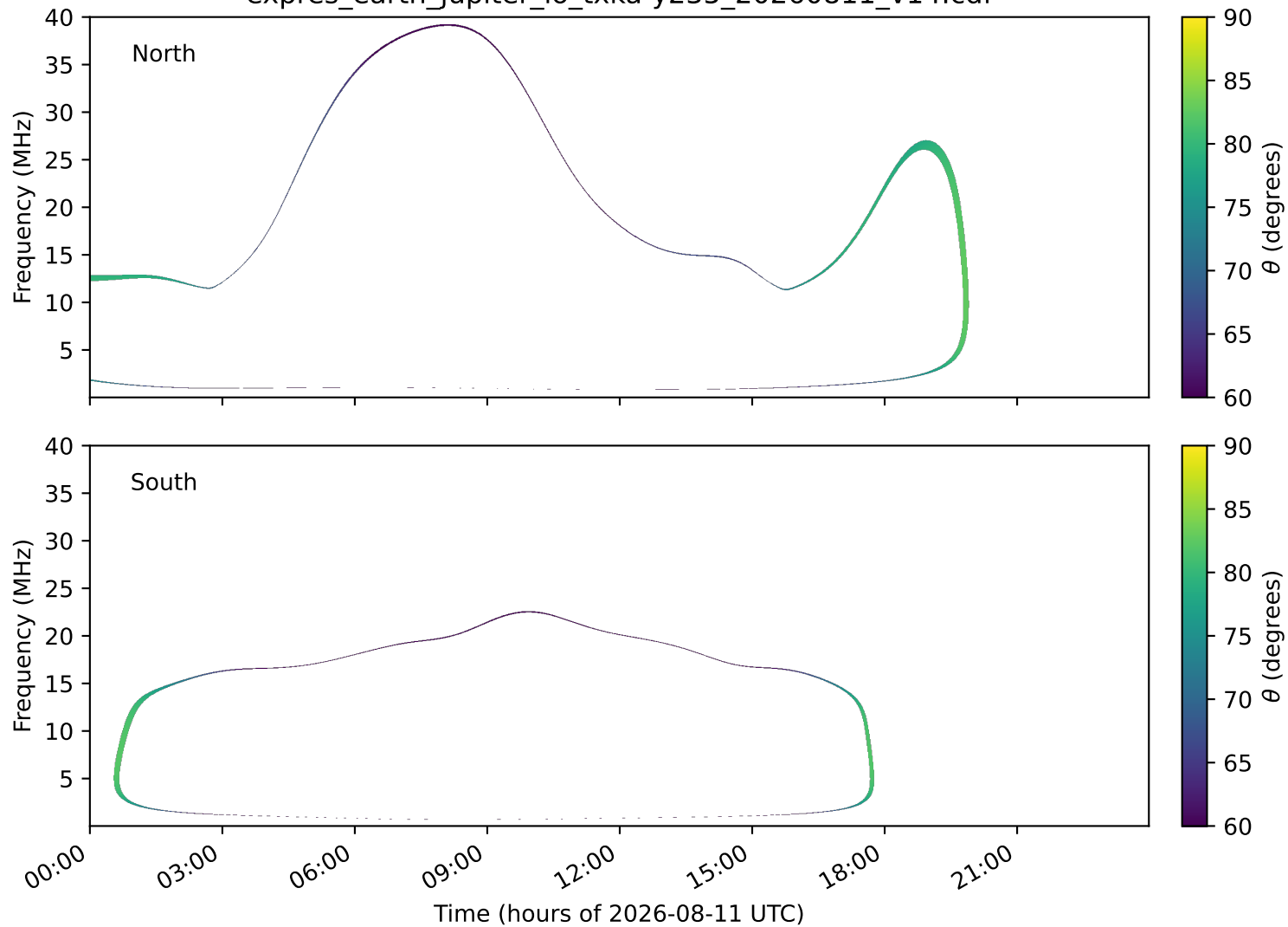
expres_earth_jupiter_io_txka-y235_20260811_v14.cdf
