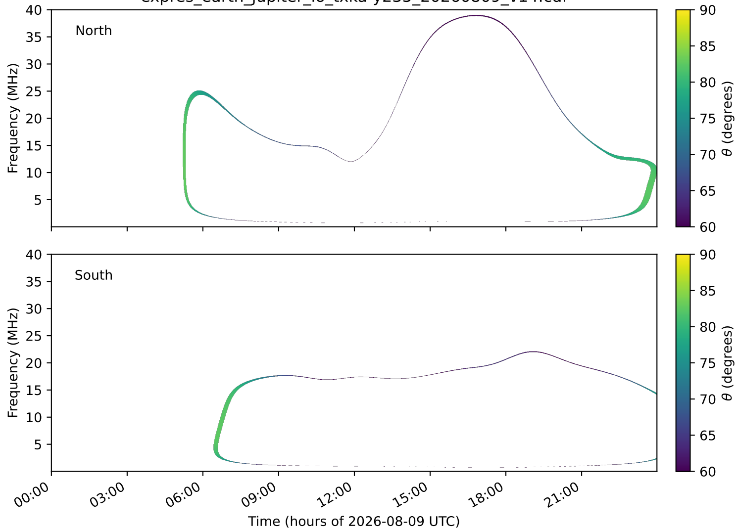
expres_earth_jupiter_io_txka-y235_20260809_v14.cdf
