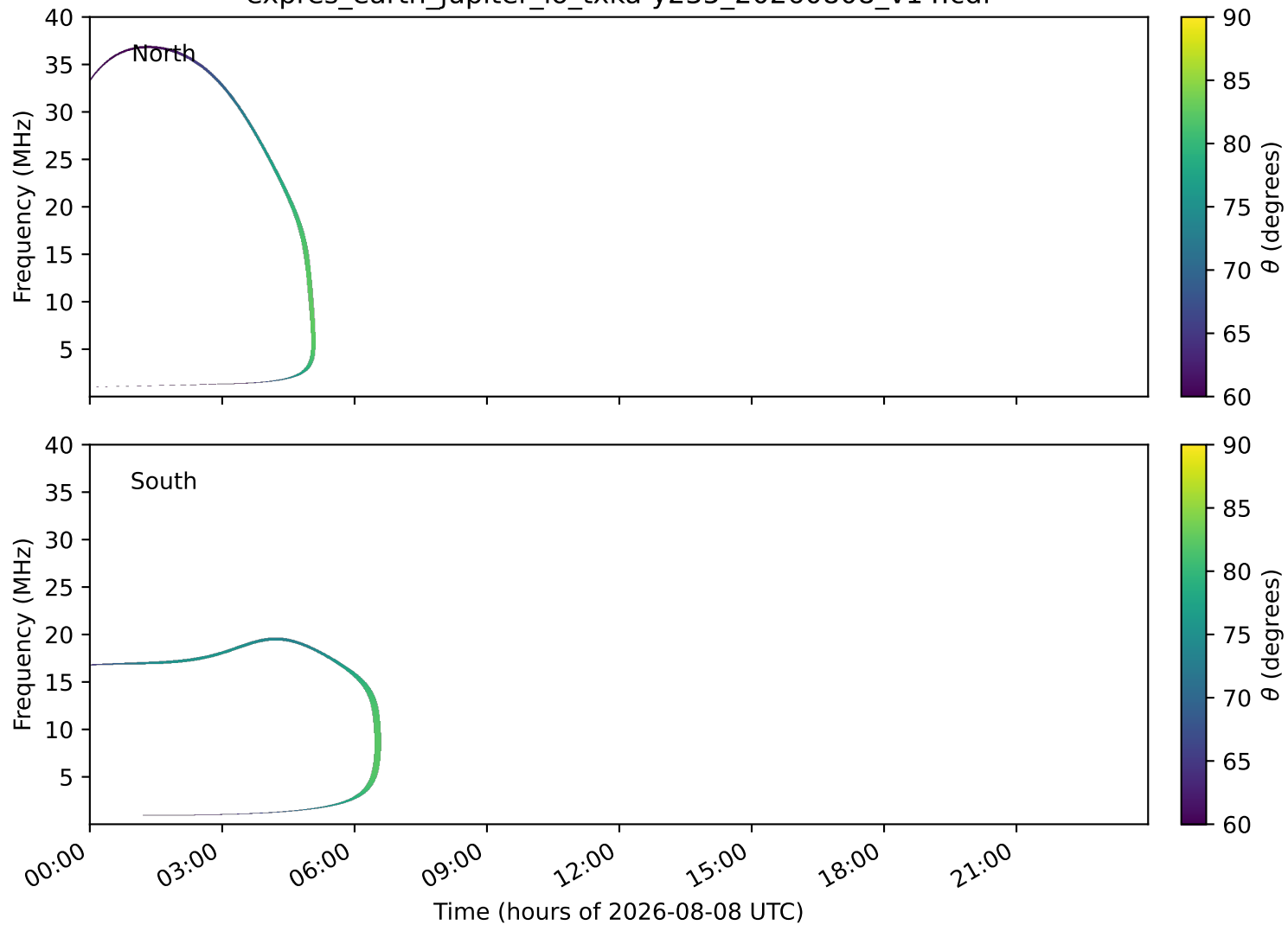
expres_earth_jupiter_io_txka-y235_20260808_v14.cdf
