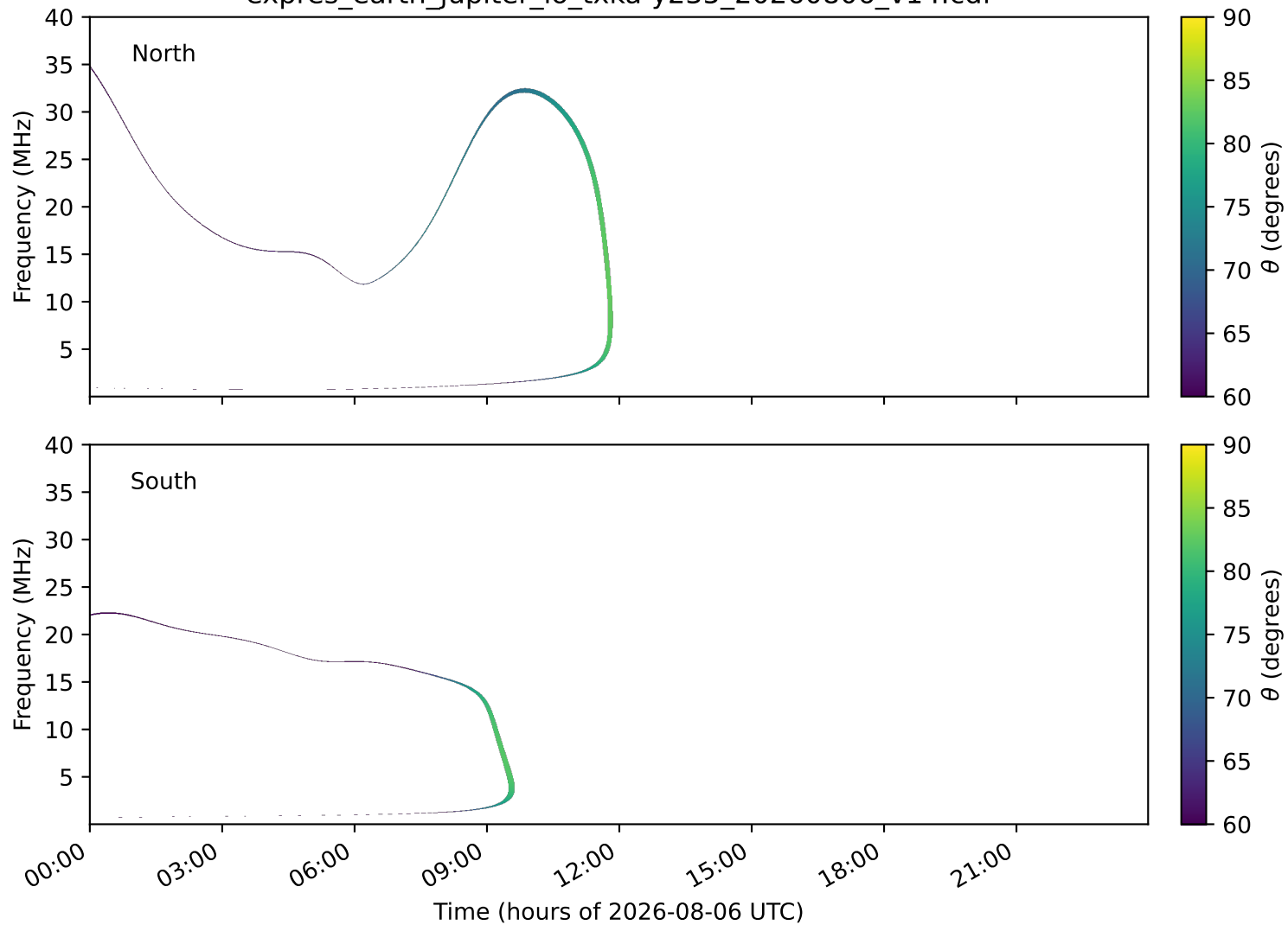
expres_earth_jupiter_io_txka-y235_20260806_v14.cdf
