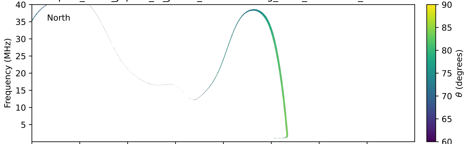
expres_earth_jupiter_io_jrm33_lossc-wid1deg_3kev_20260829_v11.cdf
