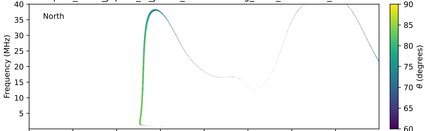
expres_earth_jupiter_io_jrm33_lossc-wid1deg_3kev_20260825_v11.cdf
