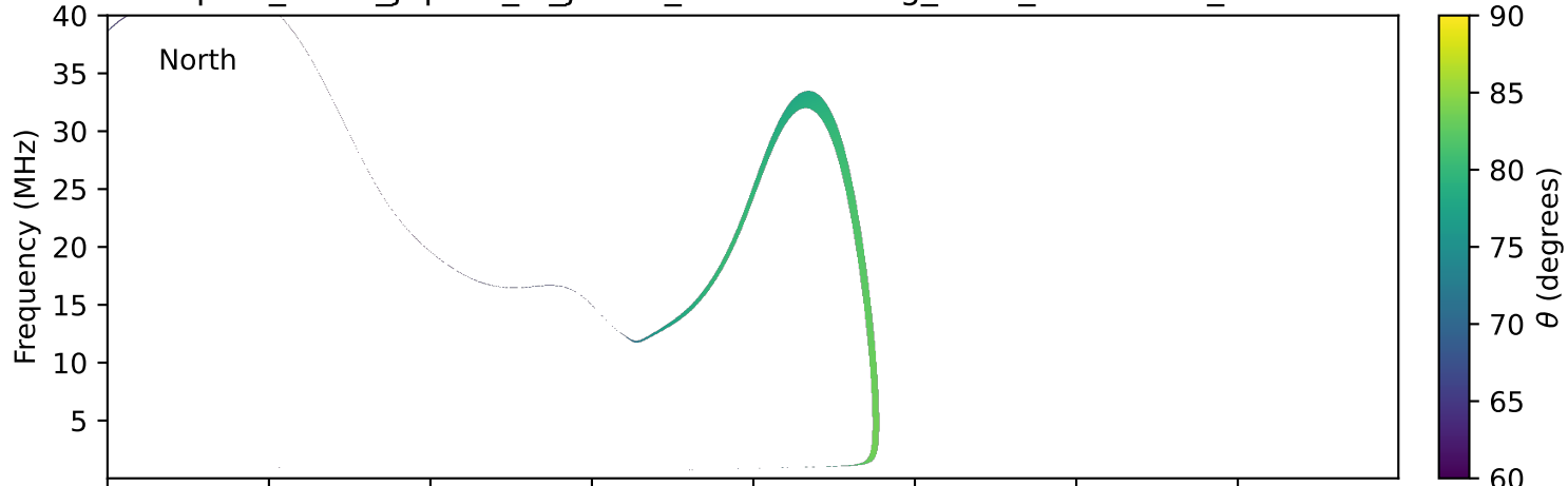
expres_earth_jupiter_io_jrm33_lossc-wid1deg_3kev_20260822_v11.cdf
