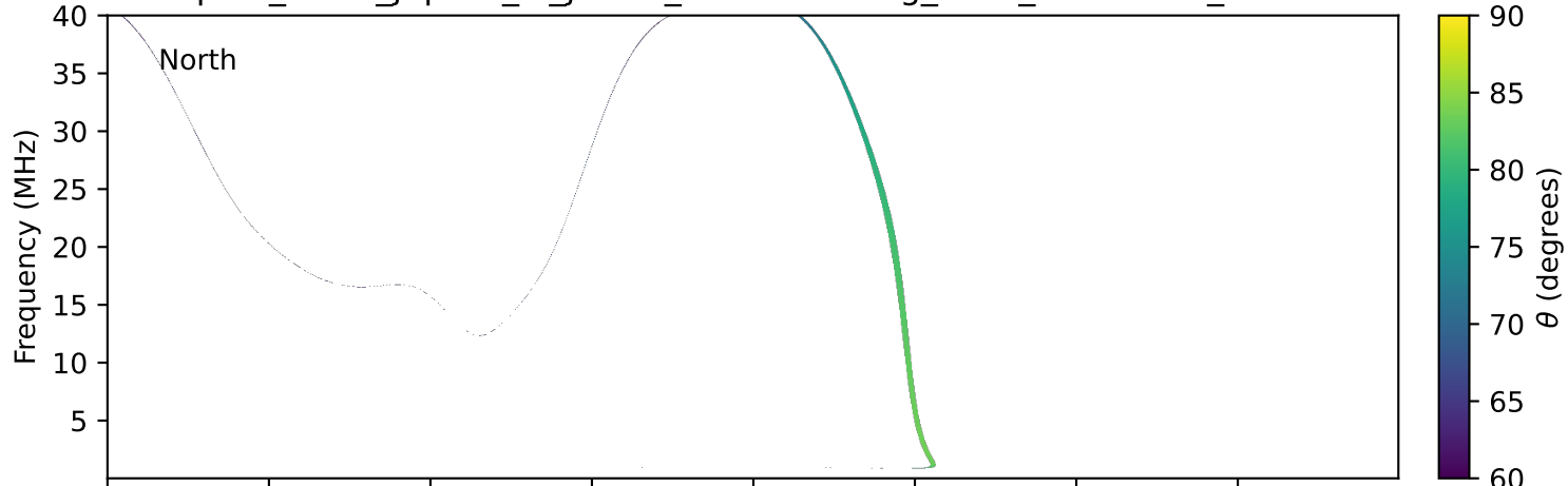
expres_earth_jupiter_io_jrm33_lossc-wid1deg_3kev_20260820_v11.cdf
