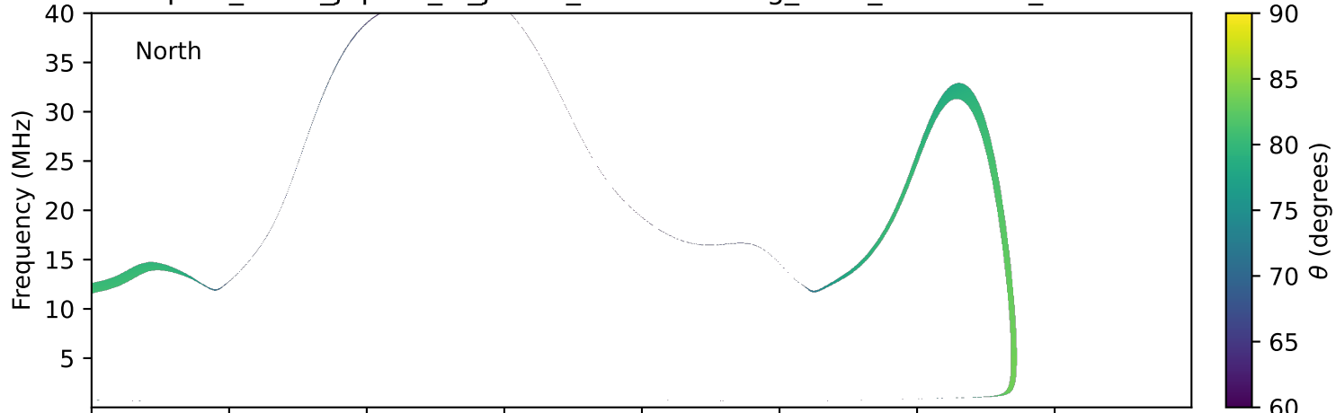
expres_earth_jupiter_io_jrm33_lossc-wid1deg_3kev_20260811_v11.cdf
