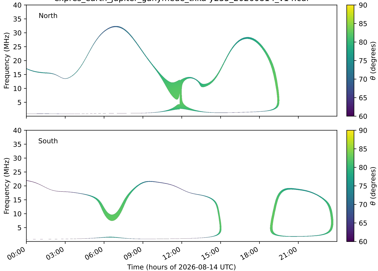
expres_earth_jupiter_ganymede_txka-y235_20260814_v14.cdf
