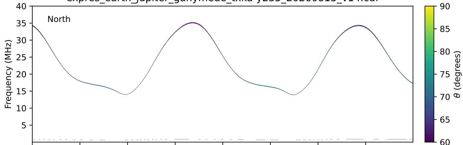
expres_earth_jupiter_ganymede_txka-y235_20260813_v14.cdf
