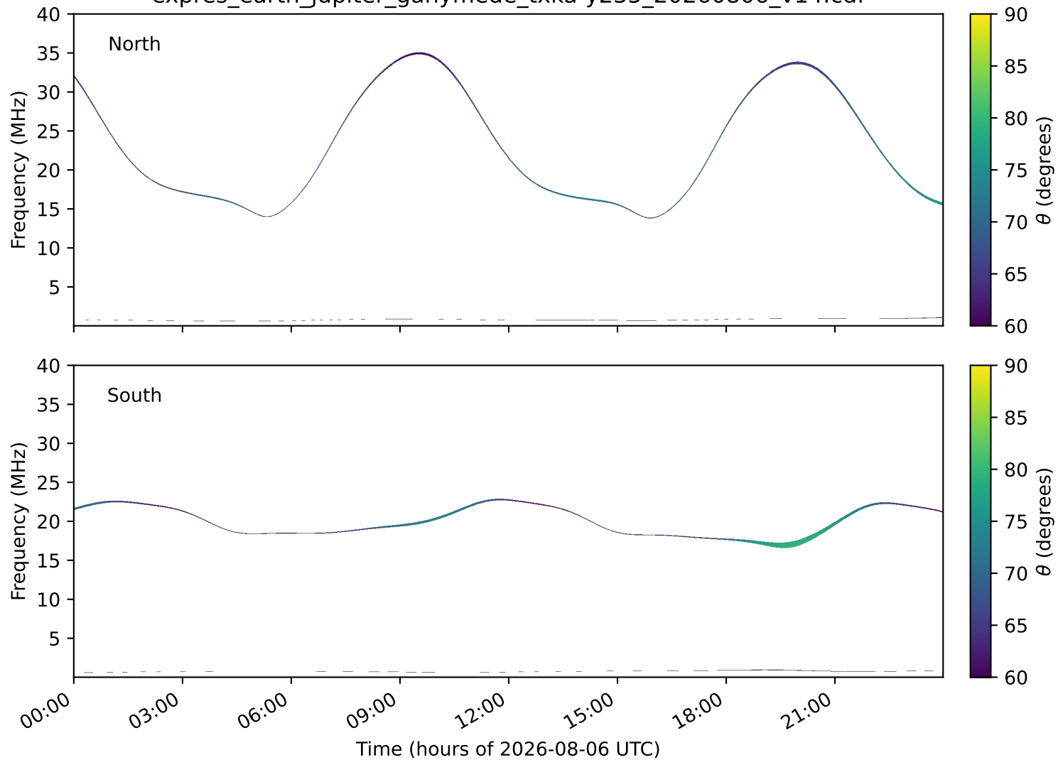
expres_earth_jupiter_ganymede_txka-y235_20260806_v14.cdf
