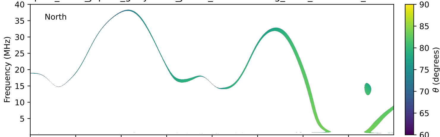
expres_earth_jupiter_ganymede_jrm33_lossc-wid1deg_3kev_20260807_v11.cdf
