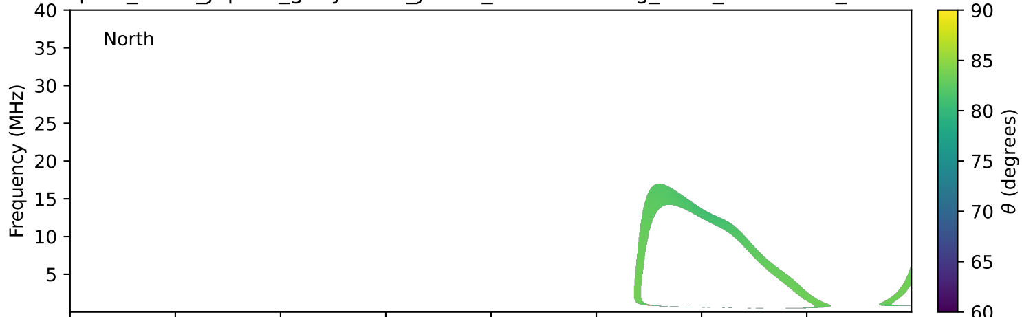
expres_earth_jupiter_ganymede_jrm33_lossc-wid1deg_3kev_20260804_v11.cdf
