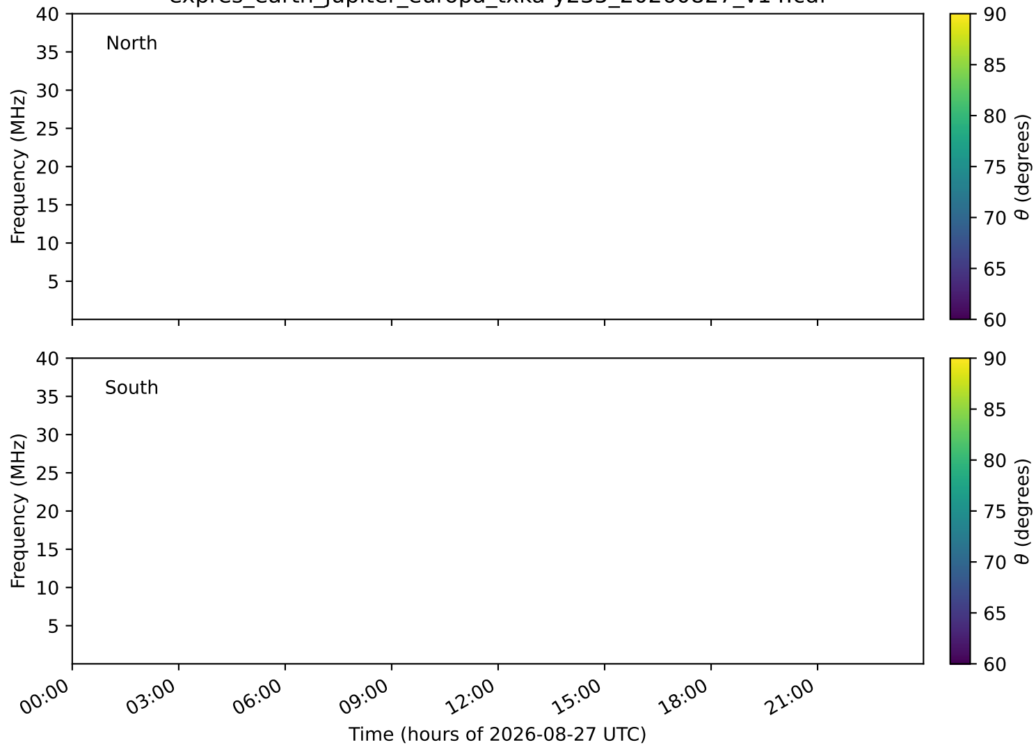
expres_earth_jupiter_europa_txka-y235_20260827_v14.cdf
