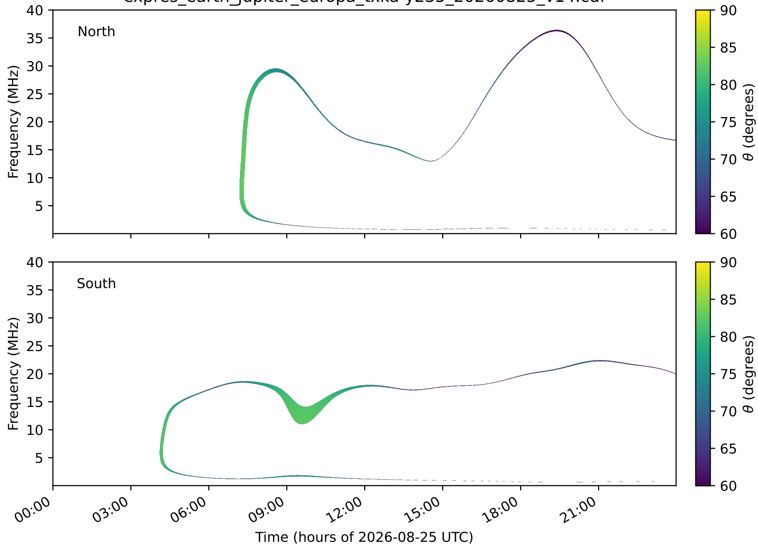
expres_earth_jupiter_europa_txka-y235_20260825_v14.cdf
