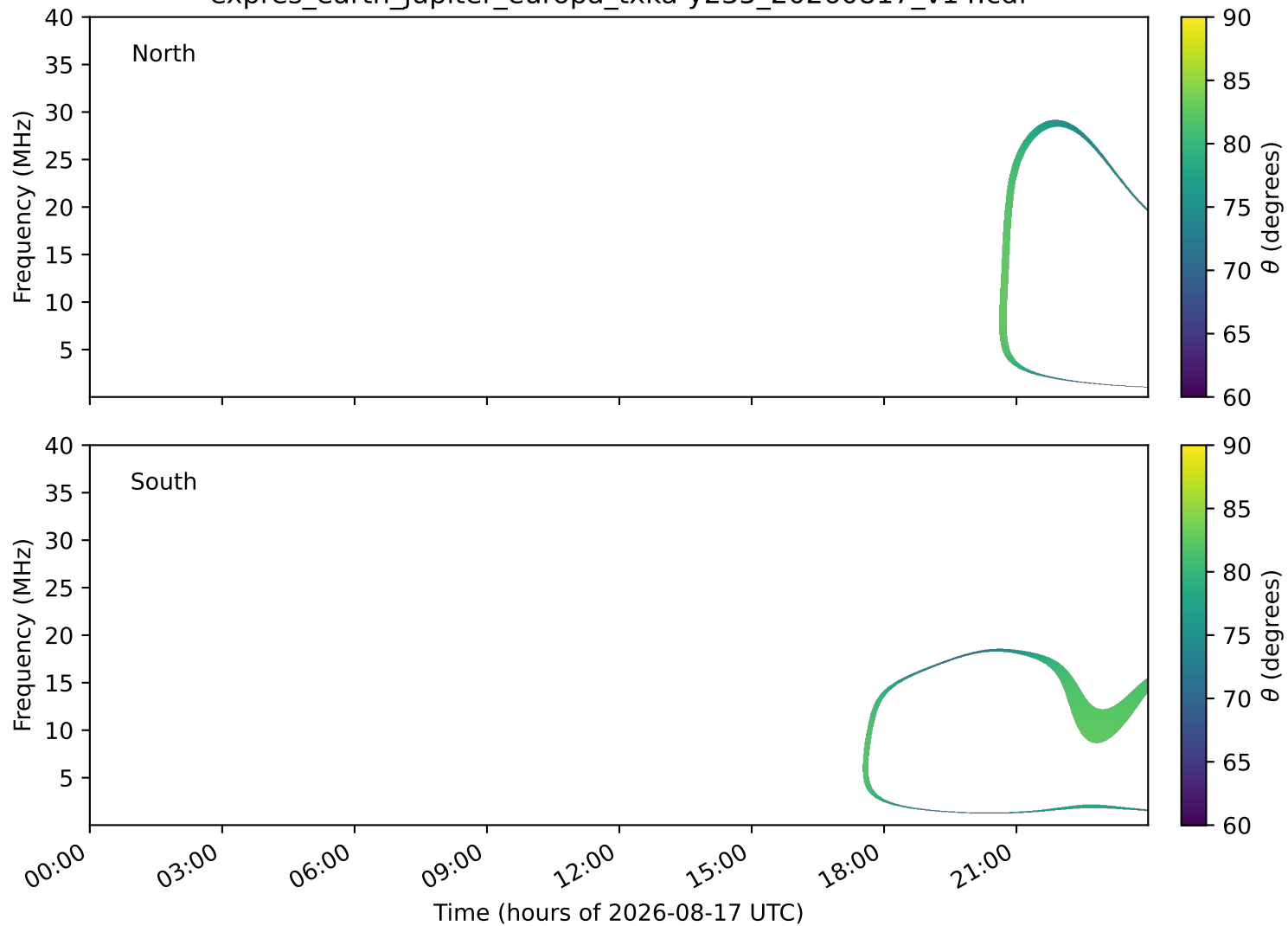
expres_earth_jupiter_europa_txka-y235_20260817_v14.cdf
